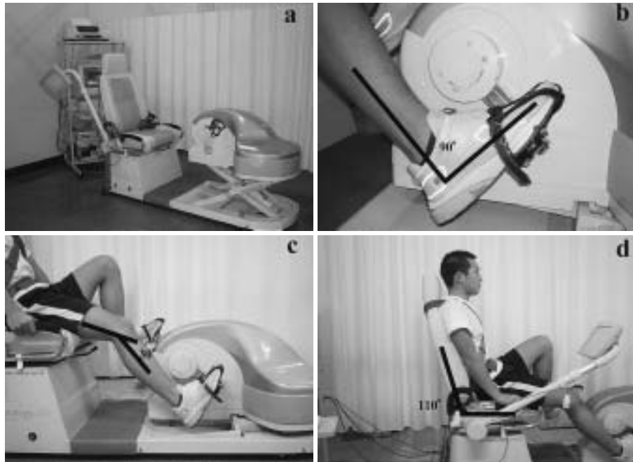
Fig. 1 Photographs showing the complete pedal-type isokinetic device StrengthErgo240™ ( SE240 ) a : Over view. b : The ankle joint is set to 90 degrees of flexion. c : Seat position is set to ensure a 30 degree of knee flexion on leg extension. d : The angle of the backrest is set at 110 degrees to the horizontal plane.
